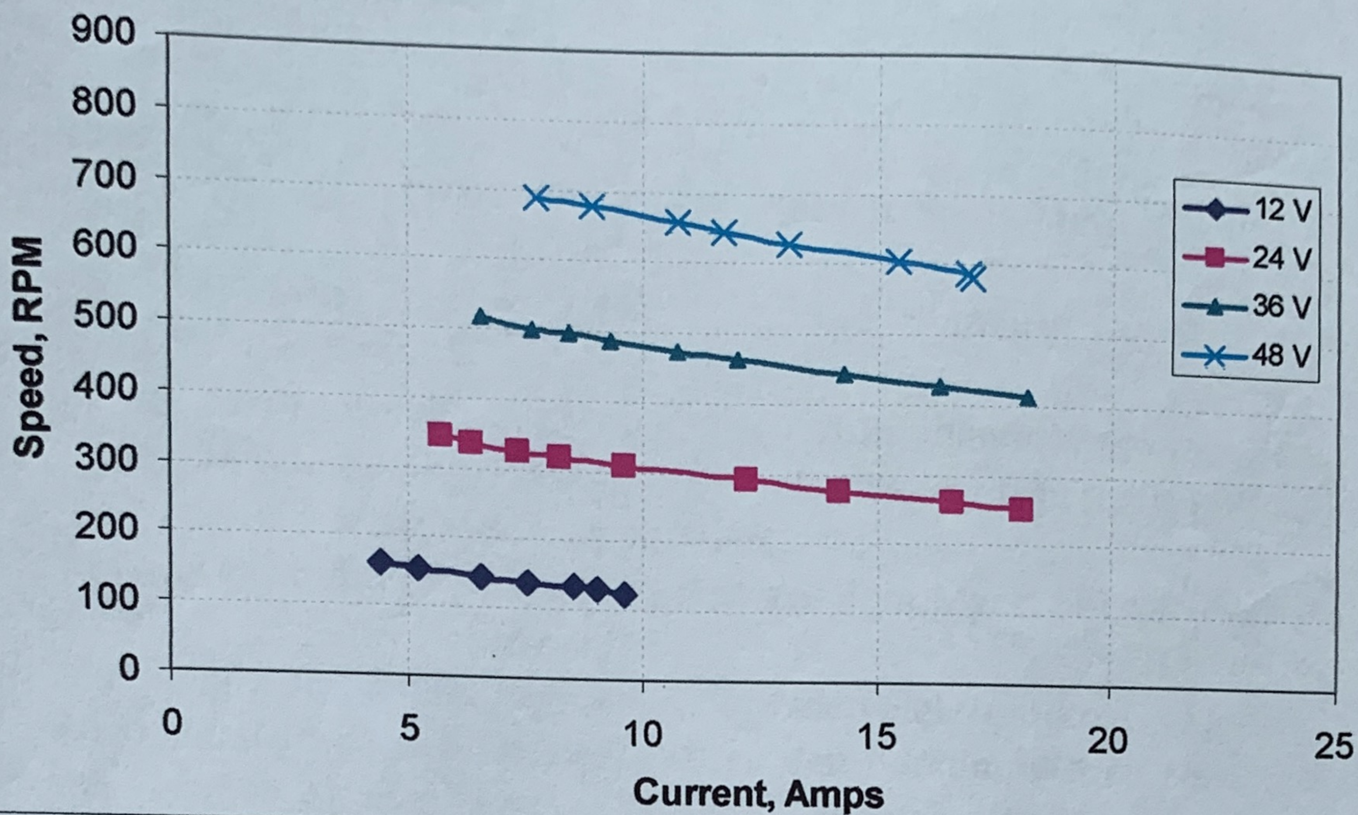
AH1200-Current Vs. Speed
