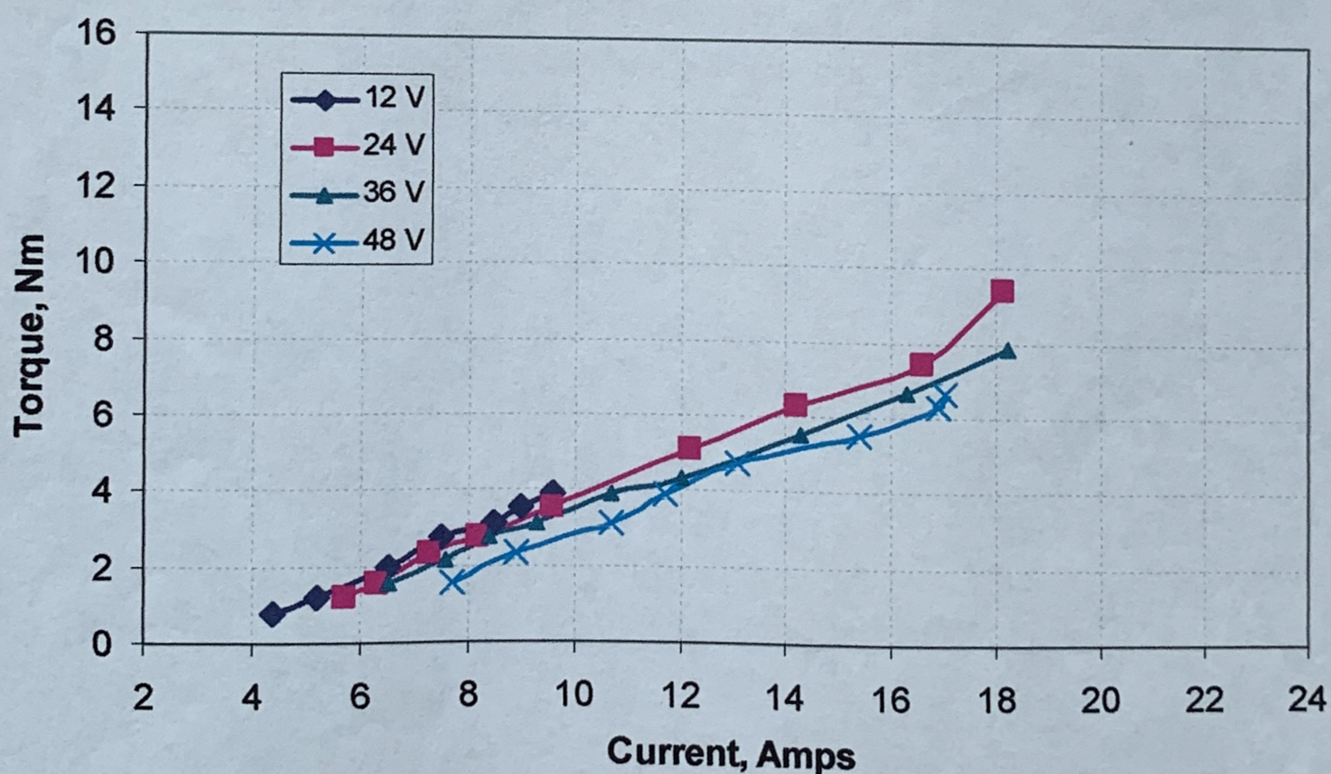
AH1200-Current Vs. Torque
